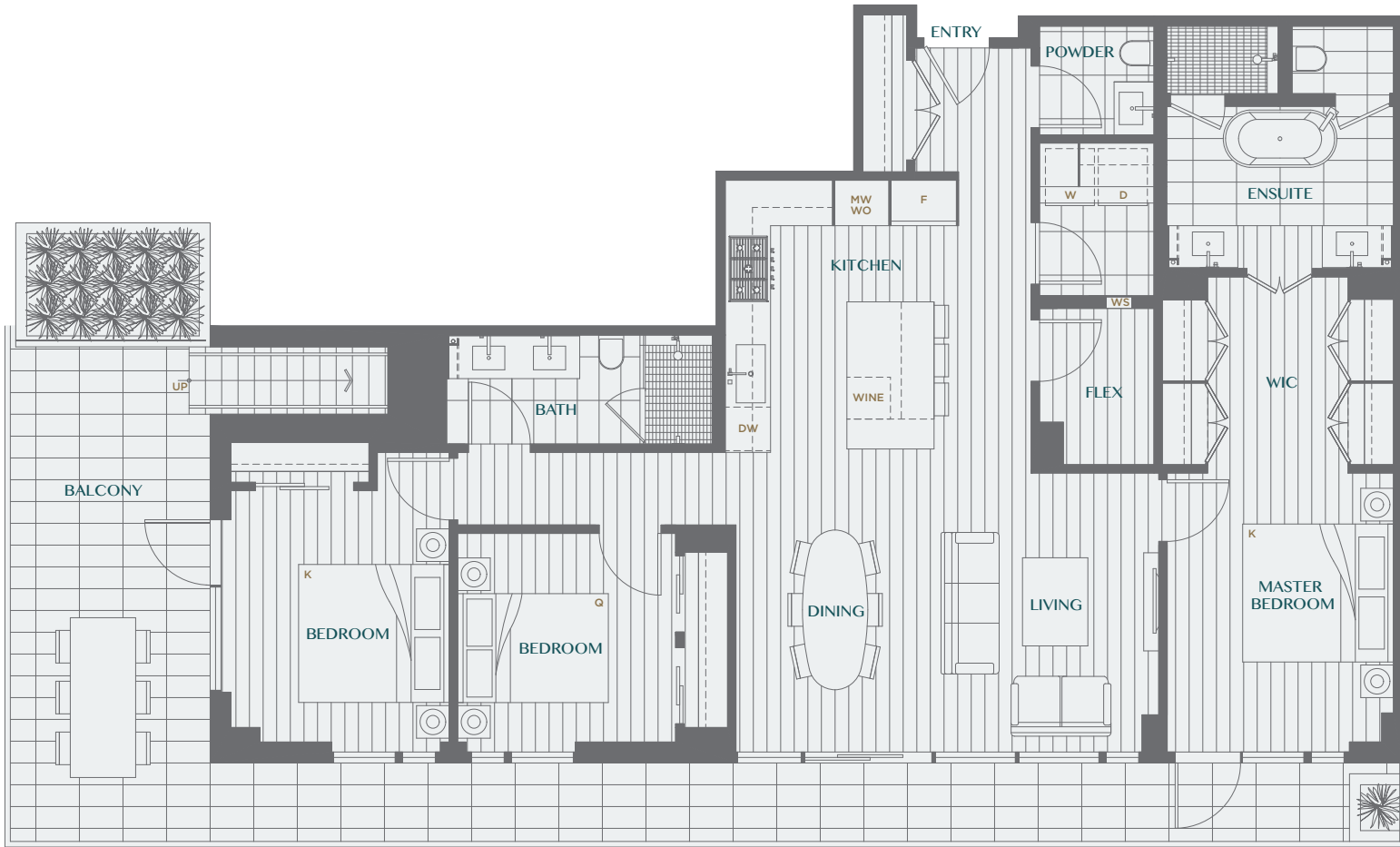
MAIN LEVEL
